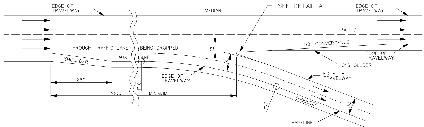
TWO LANE EXIT RAMP PAVEMENT TRANSITION Lane Drops for One and Two Lane Ramps
