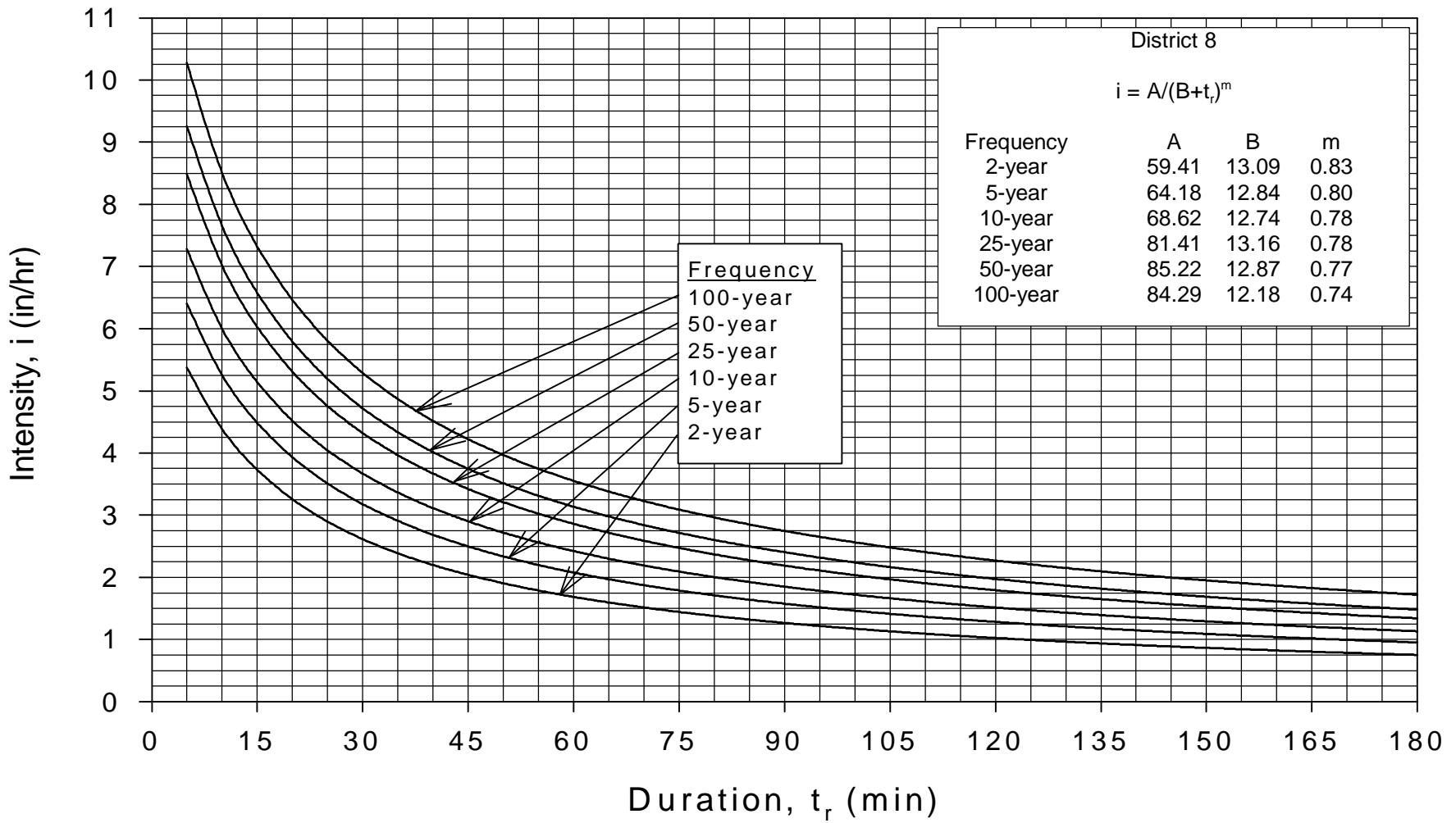
Rainfall Intensity-Duration-Frequency Curves for MoDOT District 8
