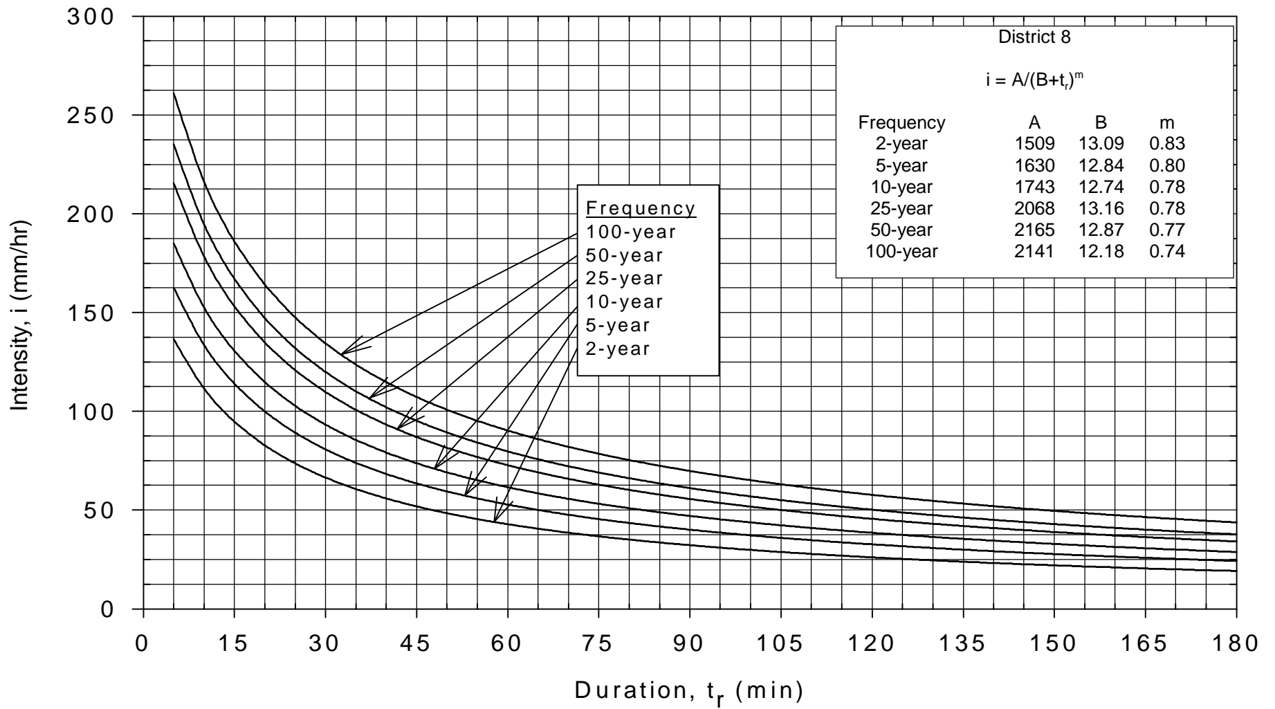
Rainfall Intensity-Duration-Frequency Curves for MoDOT District 8
