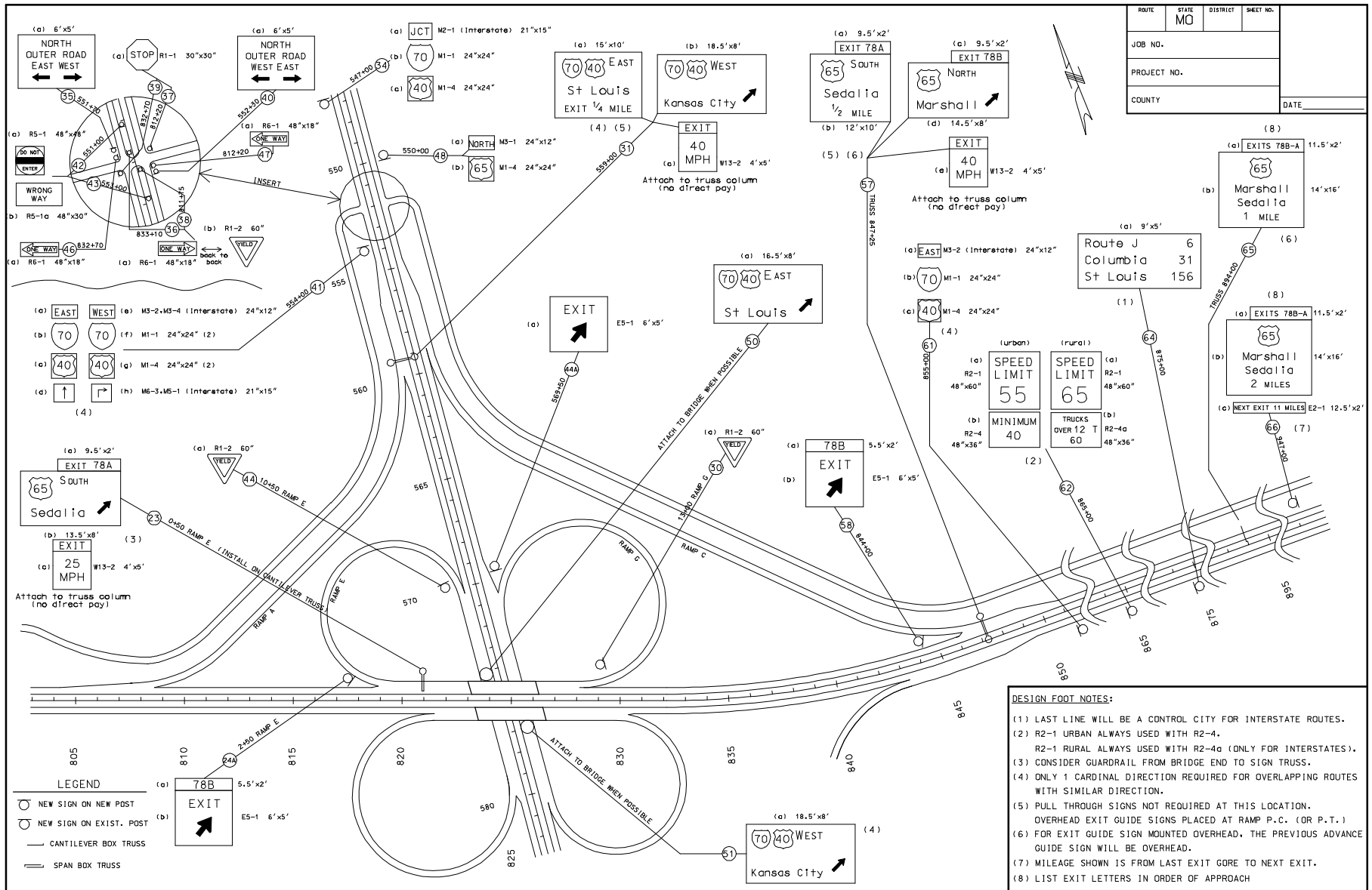
Typical Signing Plan for Cloverleaf Interchange
