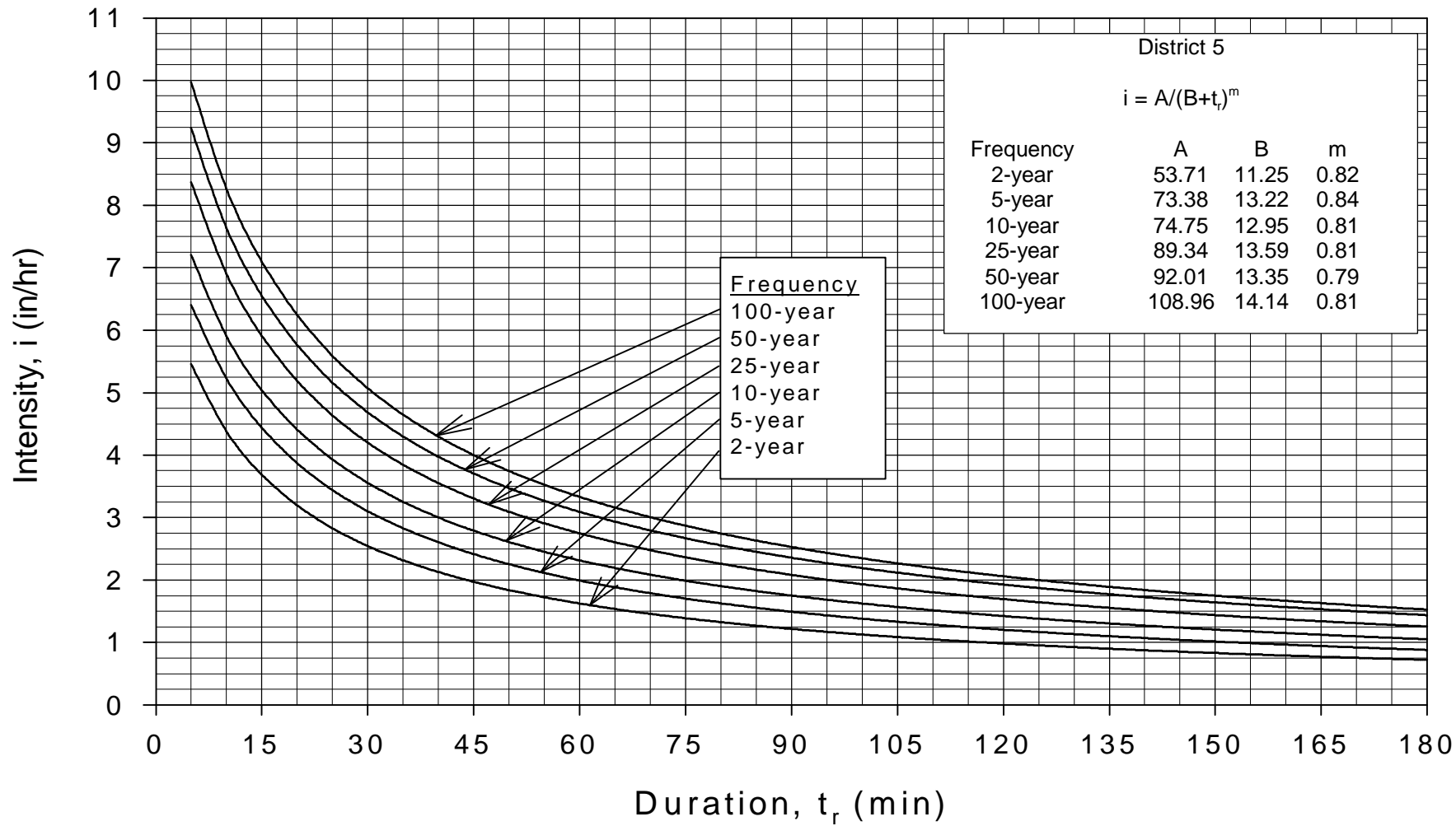
Rainfall Intensity-Duration-Frequency Curves for MoDOT District 5
