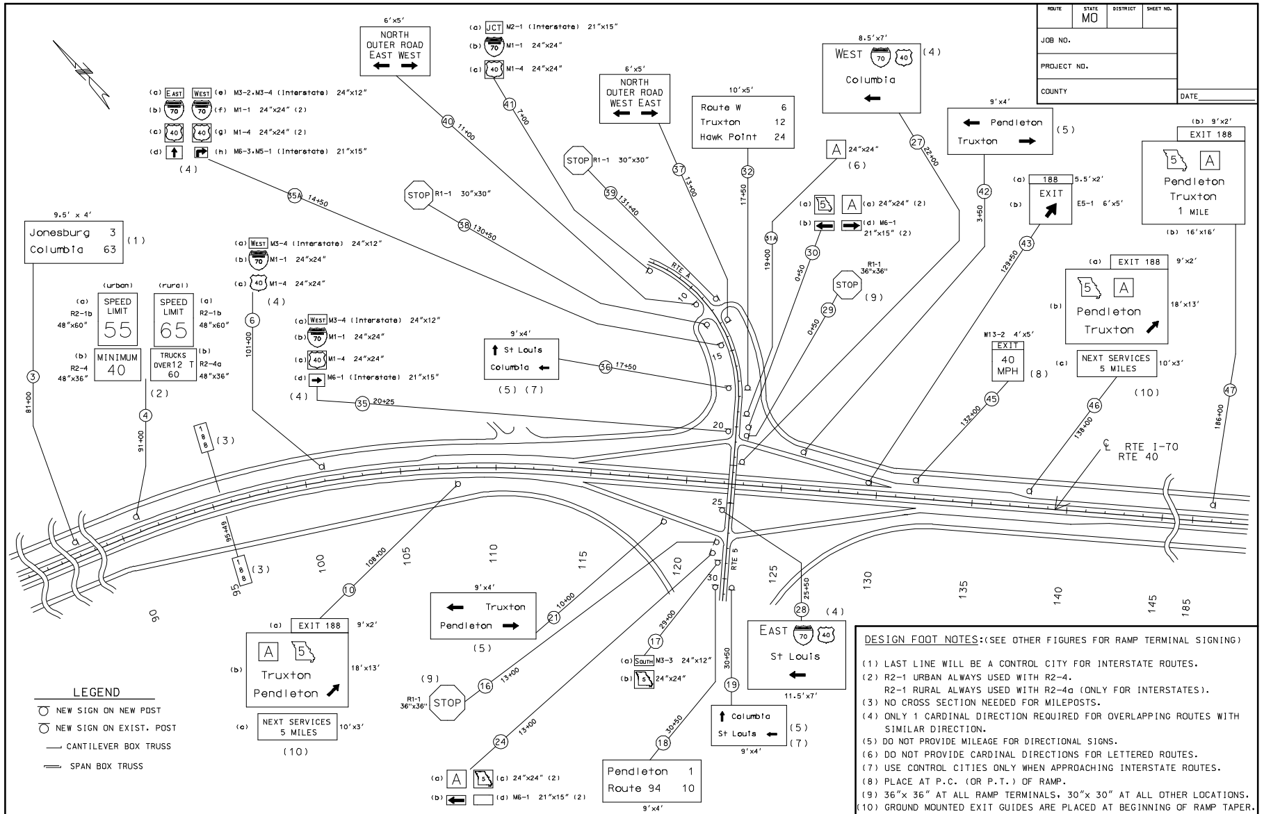
Typical Signing Plan for Diamond Interchange
