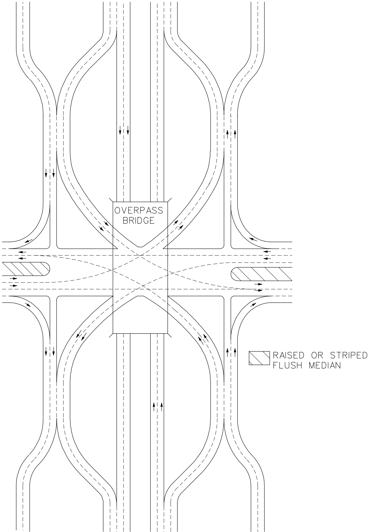
Typical Geometrics For Single Point Urban Interchanges With One-way Frontage Roads.
