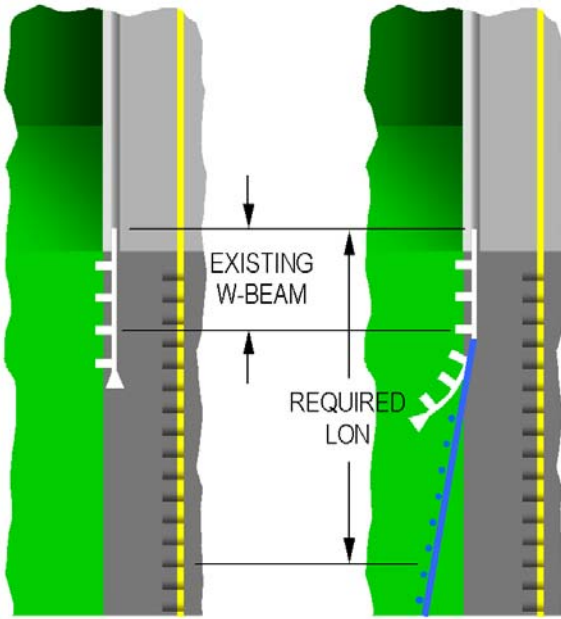
Barrier Length of Need at Median Bridge Ends
