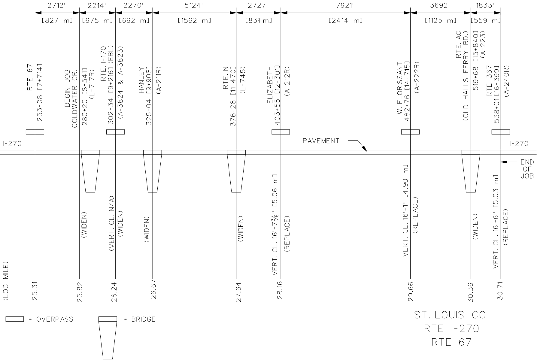
Straight Line Profile of Existing Pavement
