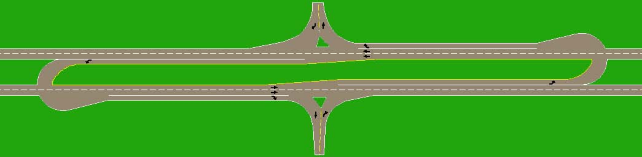
Type 4 Crossover: Directional Crossover with Median U-Turns
