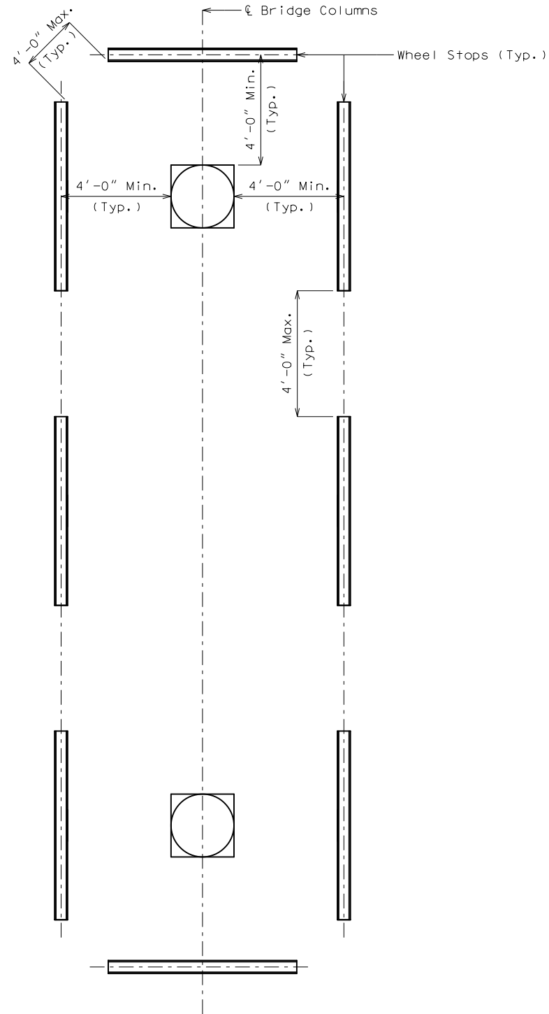
WHEEL STOP INSTALLATION DETAILS
