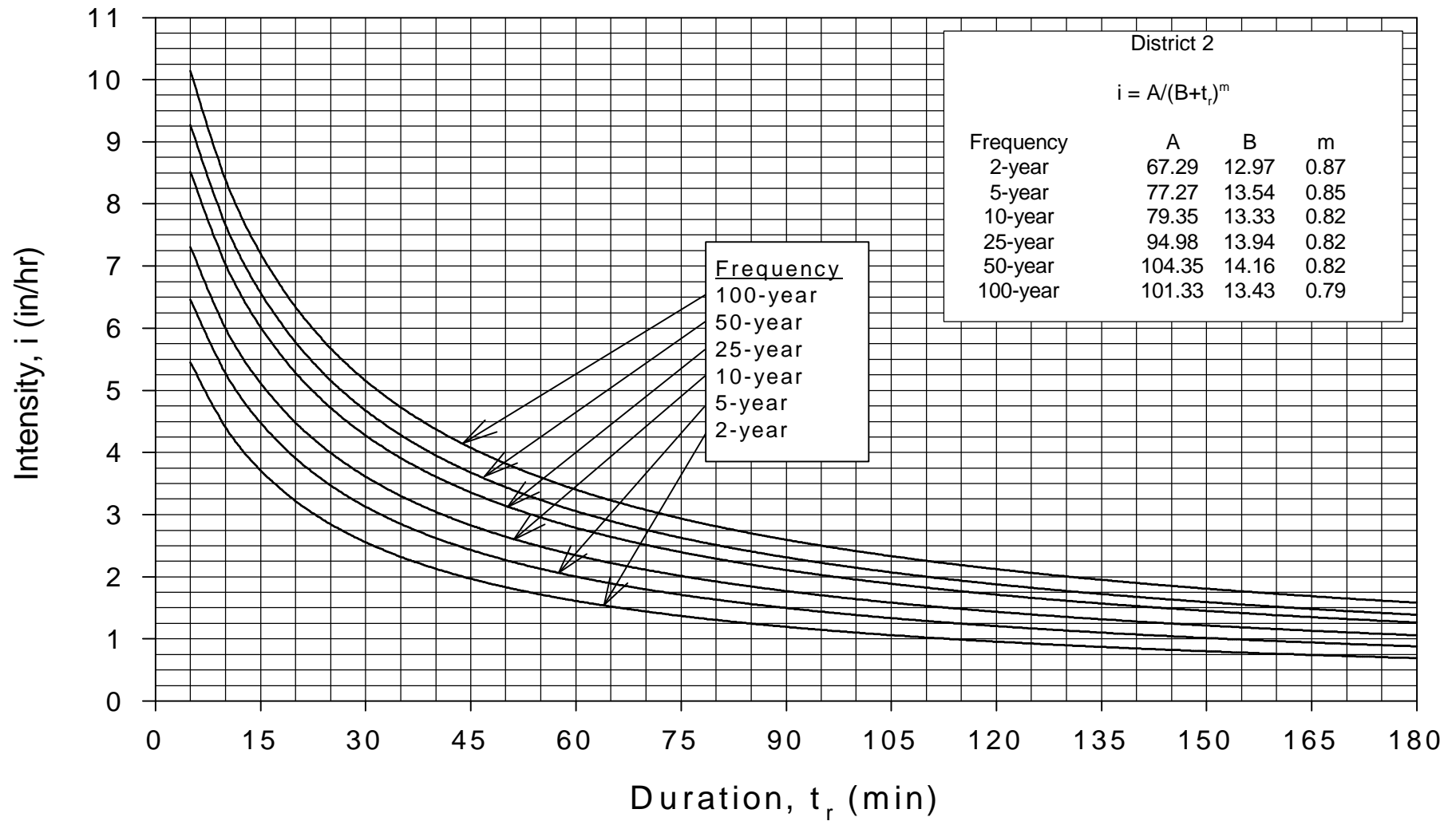
Rainfall Intensity-Duration-Frequency Curves for MoDOT District 2
