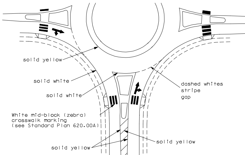
Typical Roundabout Signing and Pavement Marking
