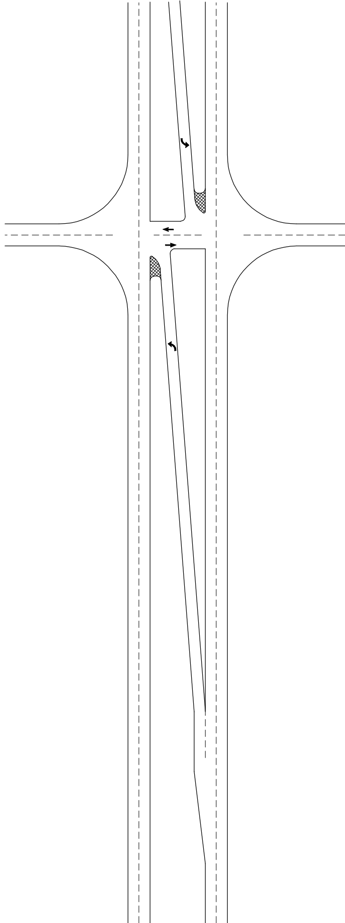
Type 3 Median Opening Offset Left Turn Lanes
