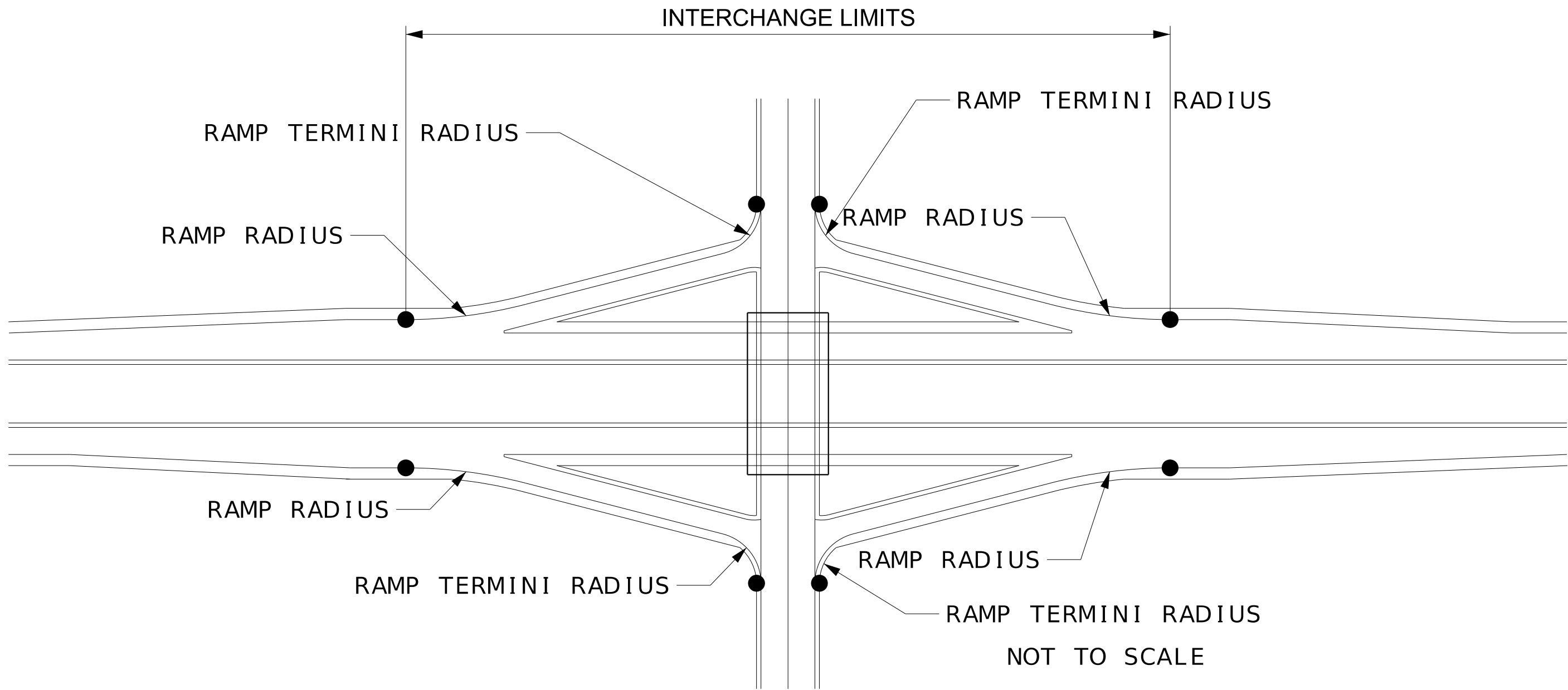
FIGURE 643.1. 1 TYPICAL INTERCHANGE LIMITS
