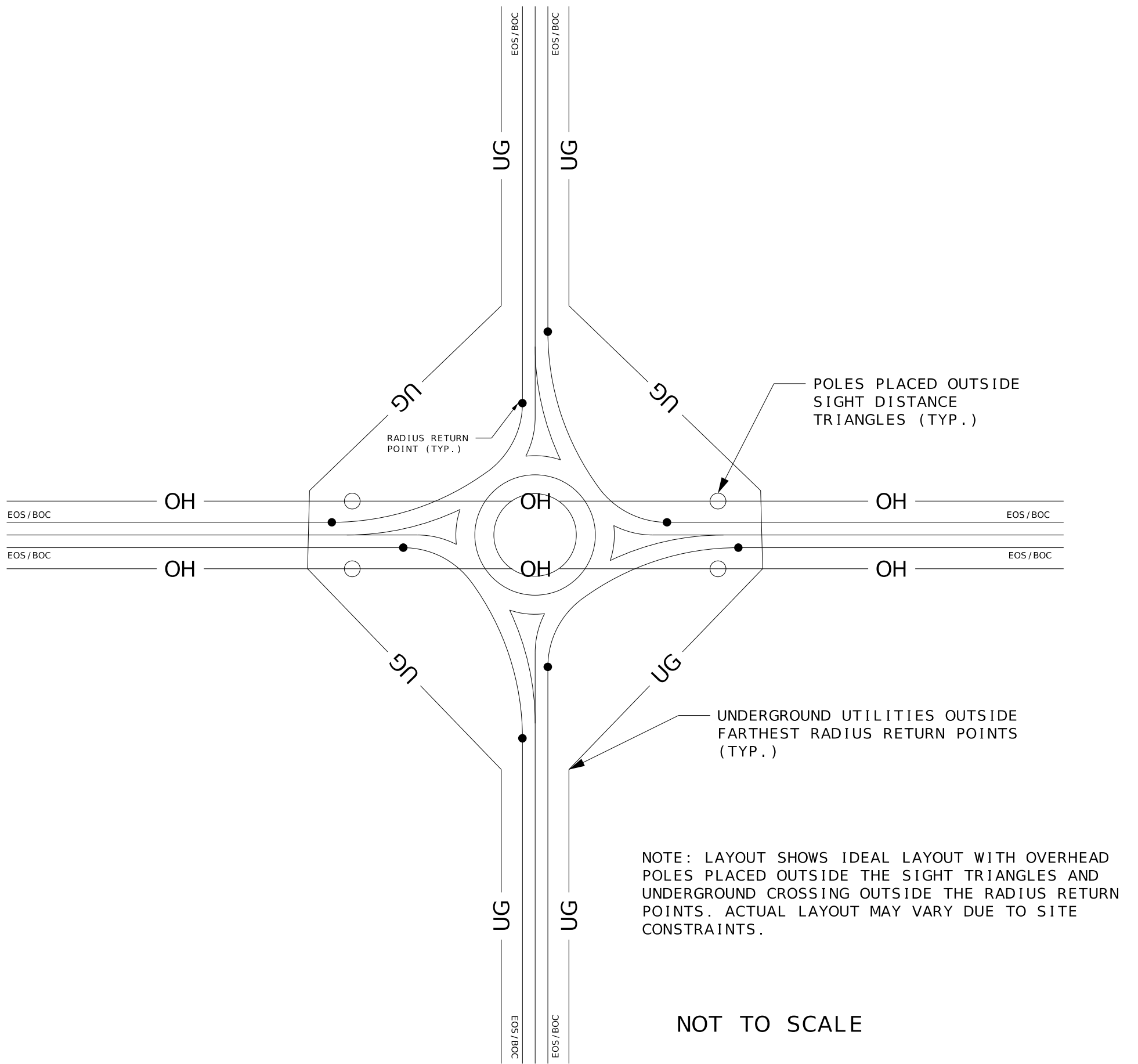
FIGURE 643.1.5 TYPICAL LOCATION OF UTILITY FACILITIES NEAR ROUNDABOUTS
